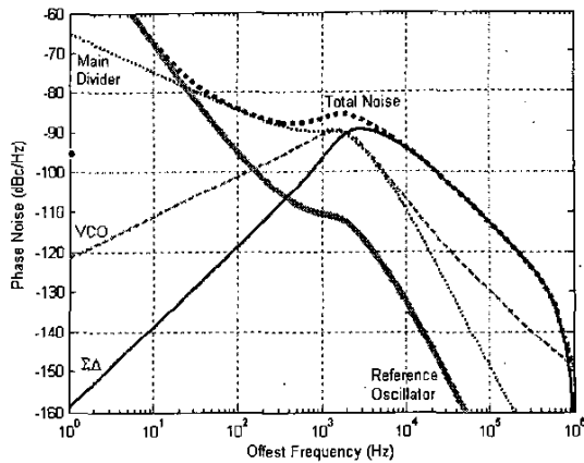
Fig. 3. Overall phase noise and its contributors
