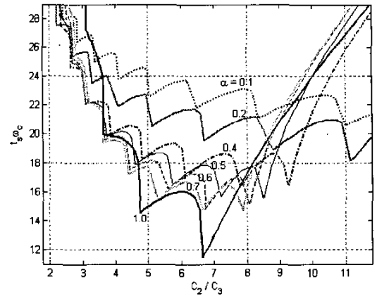
Fig. 5. Normalized settling-time against C_2/C_3 for various \alpha
